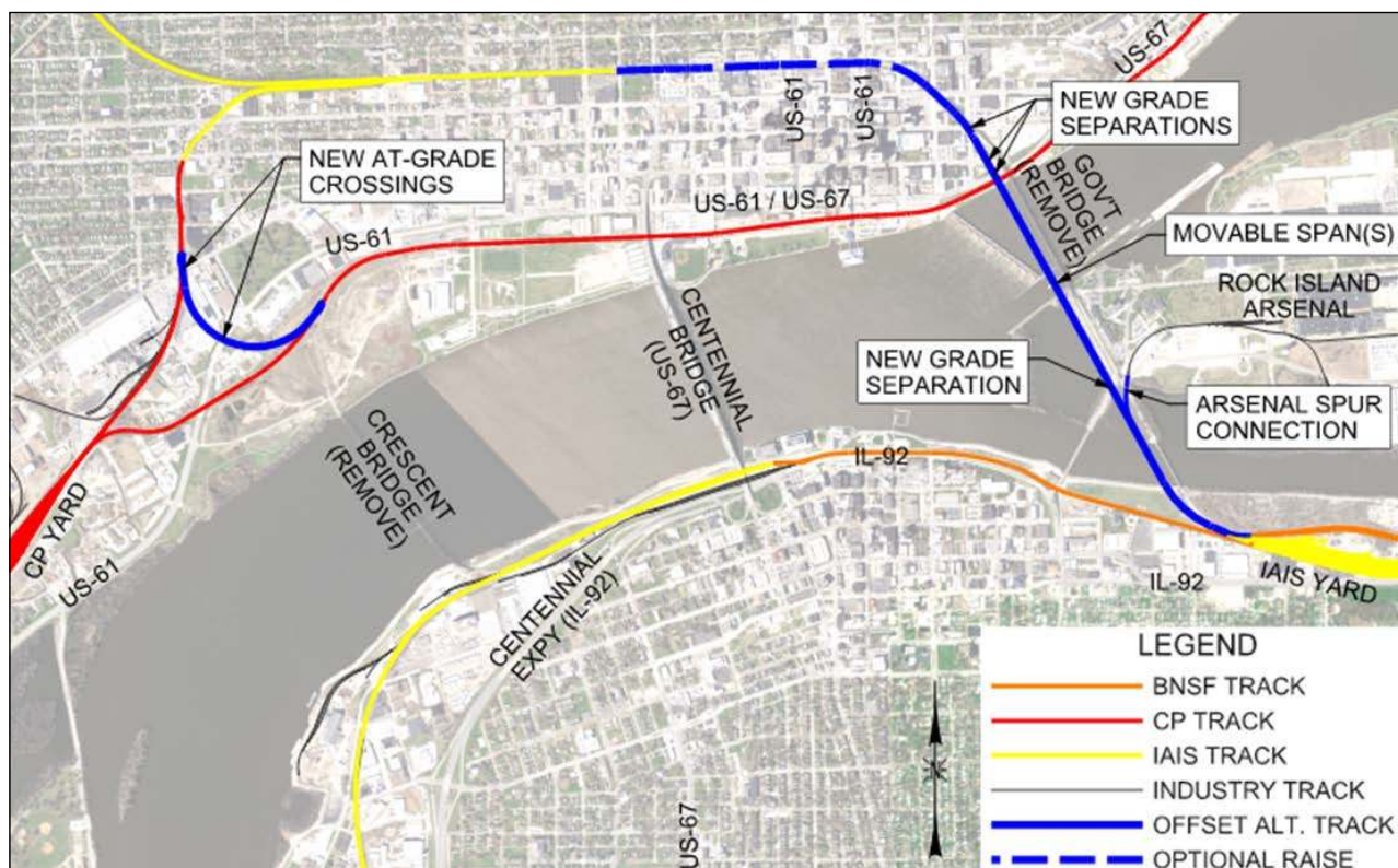
Figure 10: Central Offset Crossing Alternative
