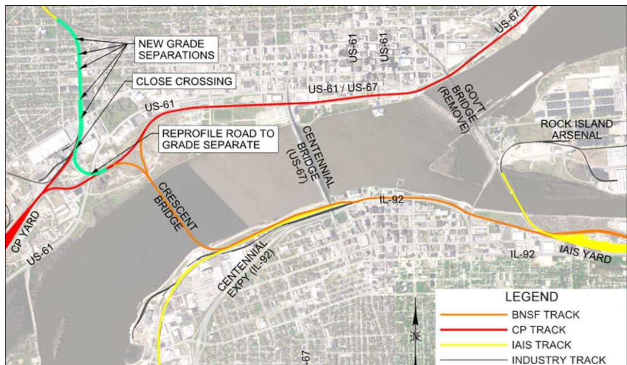
Figure 3: Crescent Bridge Only Alternative 1
