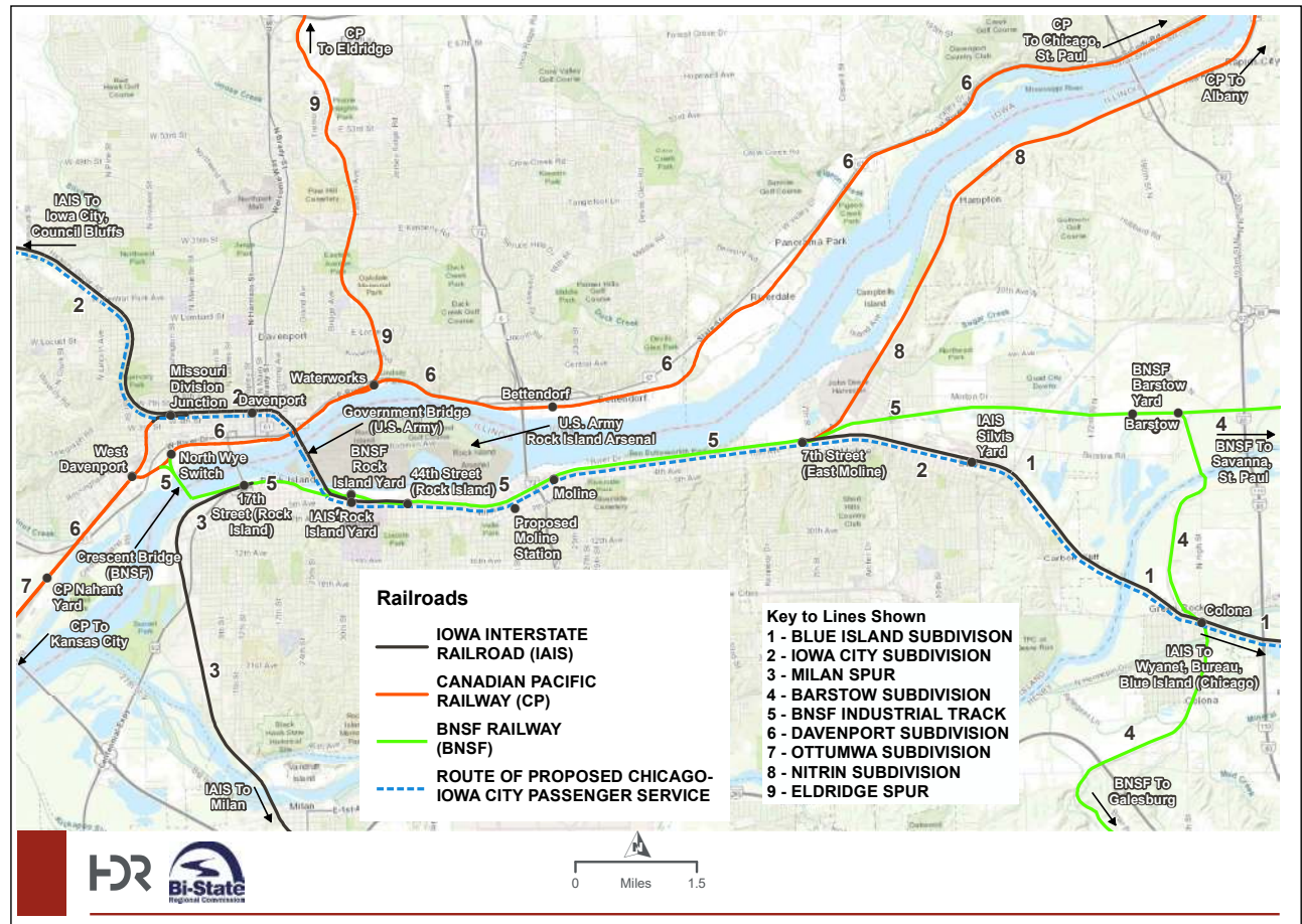
Figure 1: Existing Quad Cities Area Rail Network.
