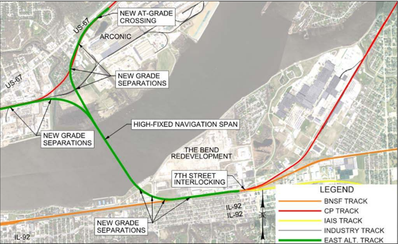
Figure 8: East Crossing Alternative
