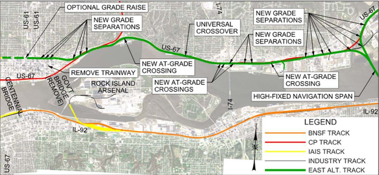
Figure 9: East Crossing Alternative CP Parallel Track
