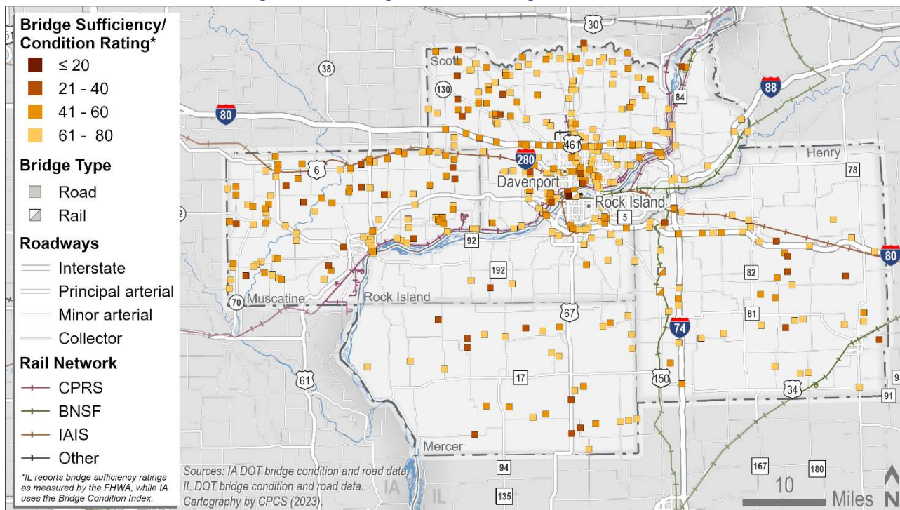
Figure 113: Bridges with a Rating under 80, 2023
